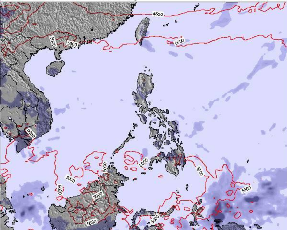
Precipitation for 3 hrs ending Sunday 14 May at 2pm PST Freezing level contours
