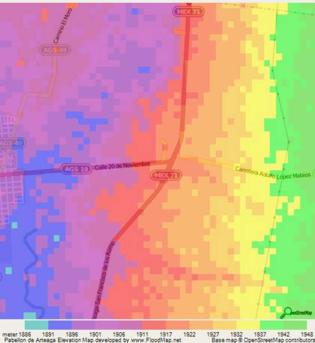
Pabellon de Arteaga Elevation: 1923 meter Map by www.FloodMap.net (beta)
