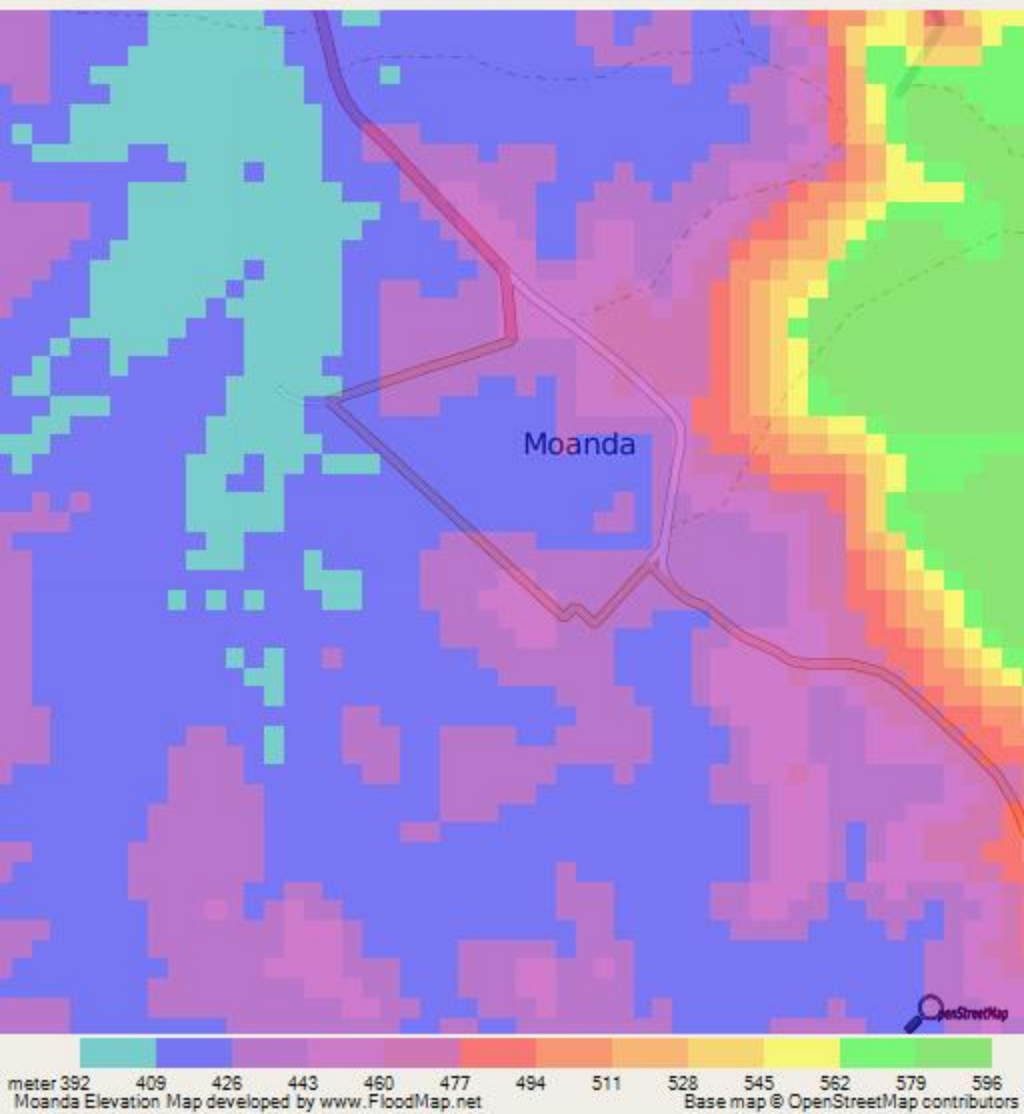
Moanda Elevation: 317 meter Map by www.FloodMap.net (beta)
