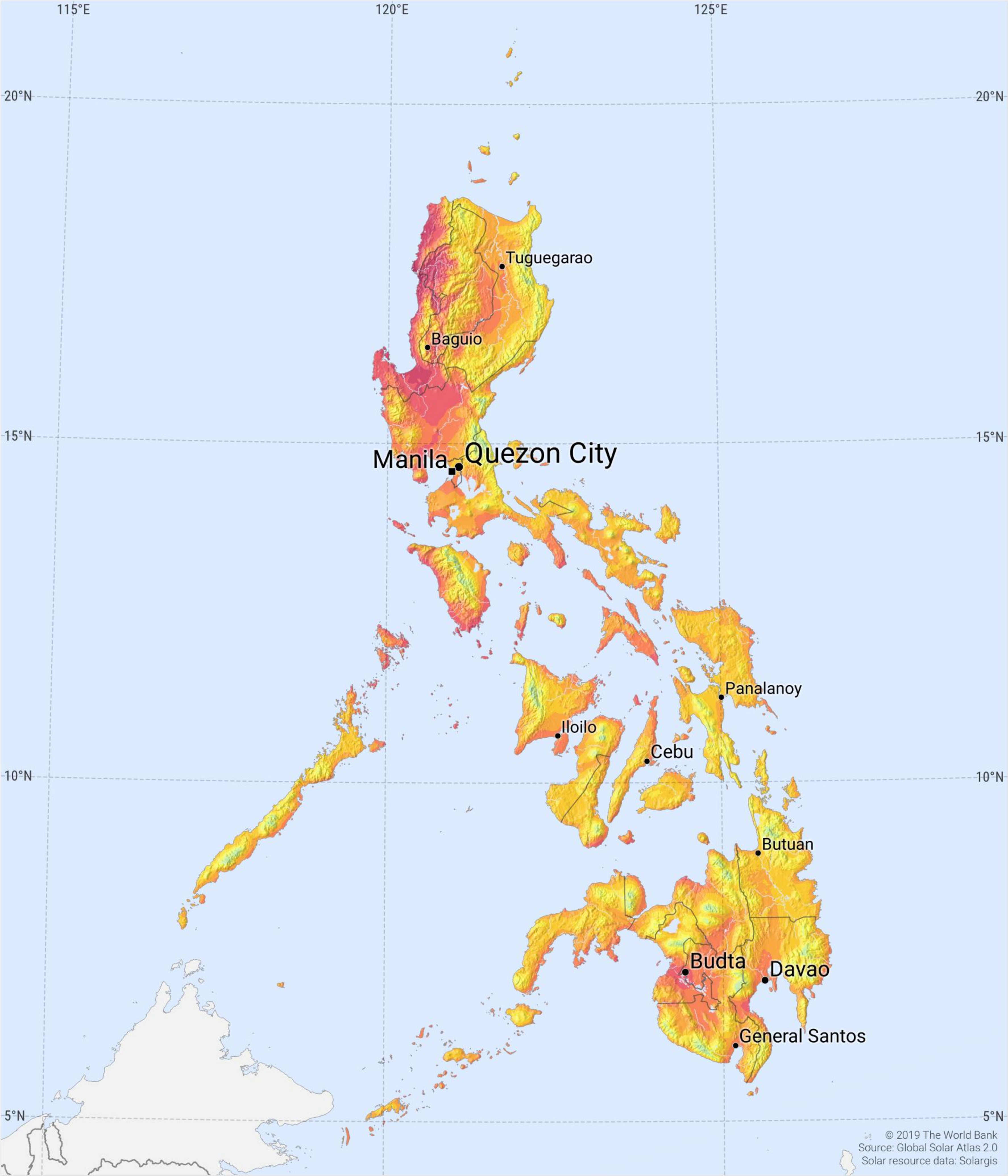
Long term average of PVOUT, period 2007-2018
